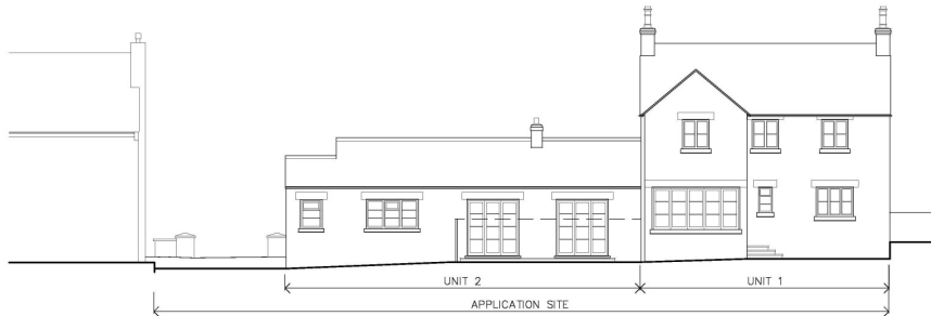
PROPOSED SOUTH ELEVATION – UNITS 1 & 2
