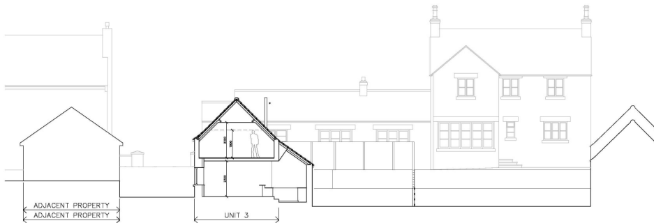
PROPOSED SECTION ON A-A • Back omitted for pipe to Unit 2
